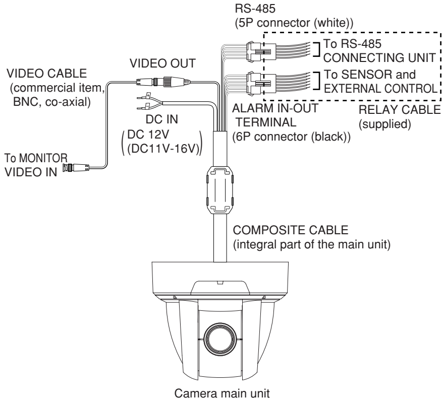
RS-485 terminal (5P connector (white))
